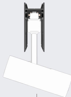
Spotlight with Crossover adapter inserted into CORE11 double emission
