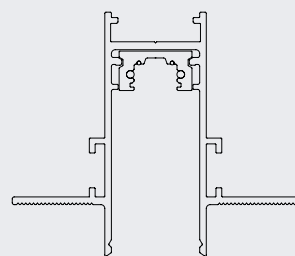
Cover M5
