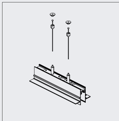
Trimless tracks
